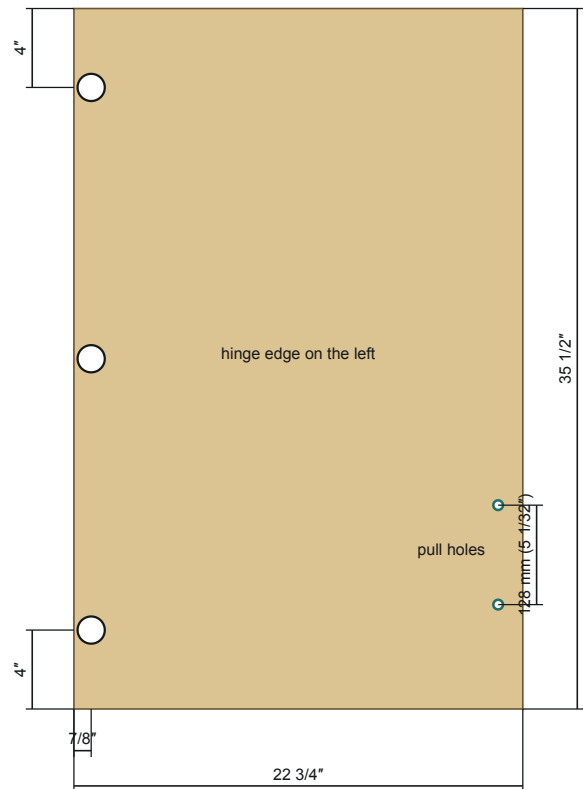
DETAIL 3 FREEZER DOOR D1, back face, hinge bores (joint J7)
