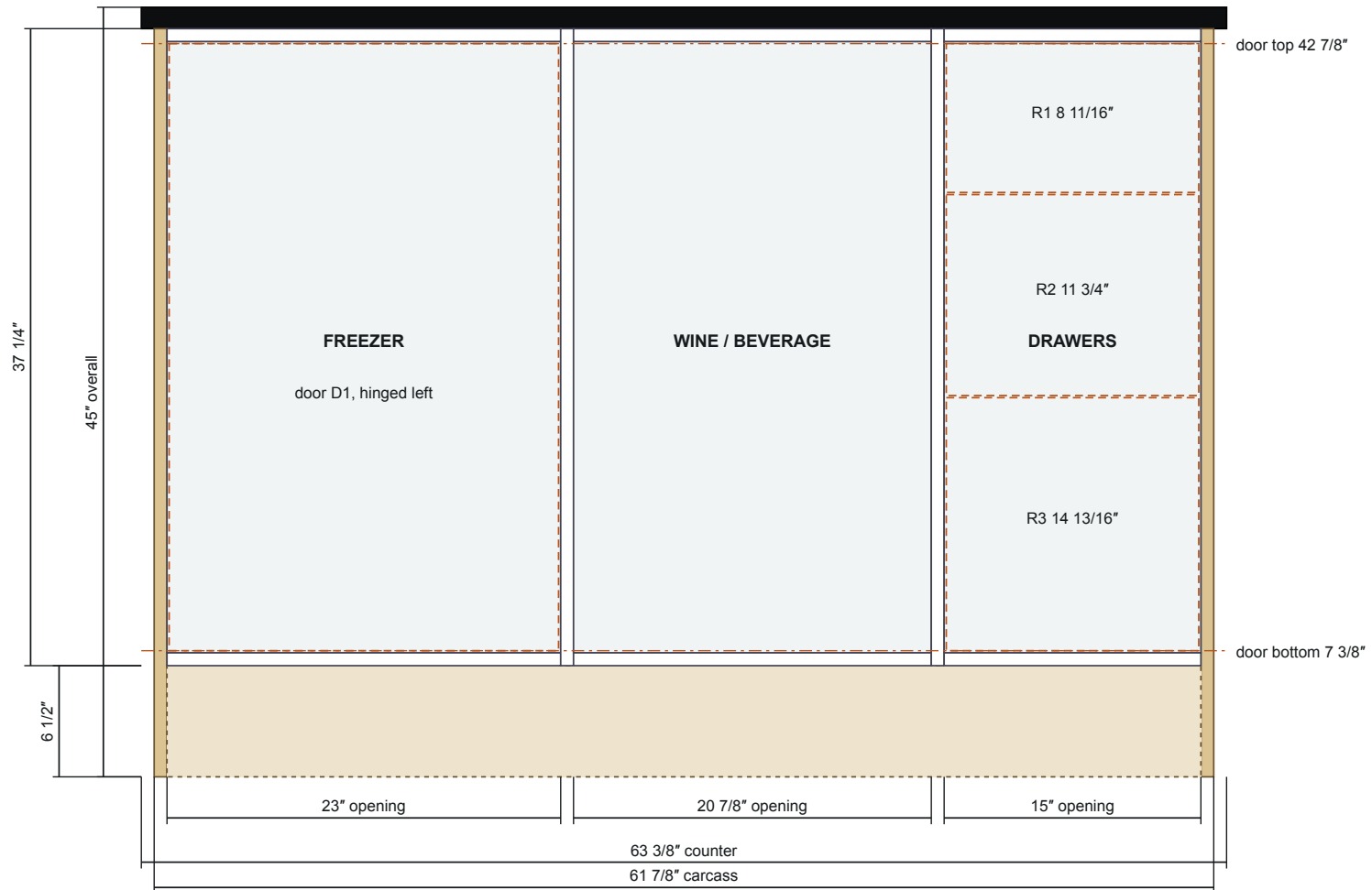
FIGURE 1 FRONT ELEVATION
