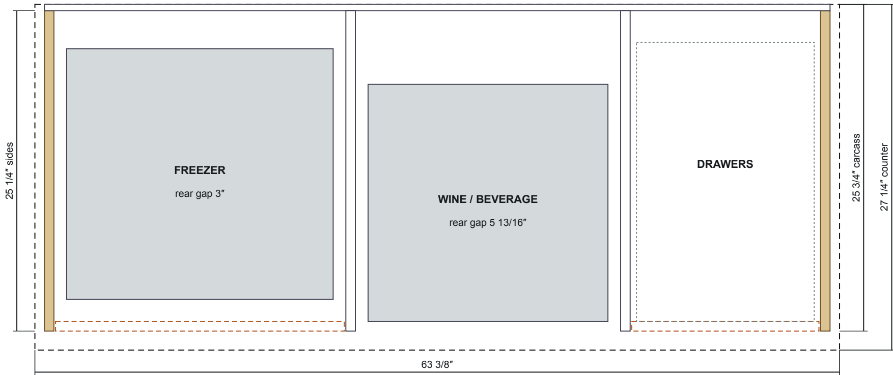
FIGURE 2 PLAN (counter removed)
