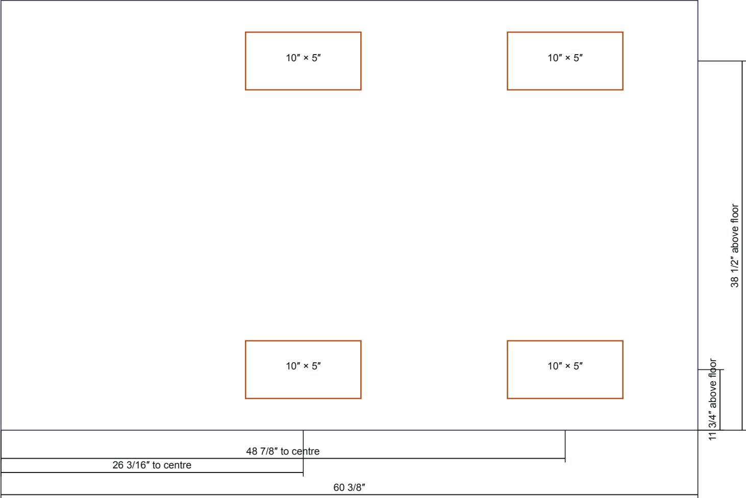
FIGURE 4 BACK ELEVATION, vent openings (seen from the back)
