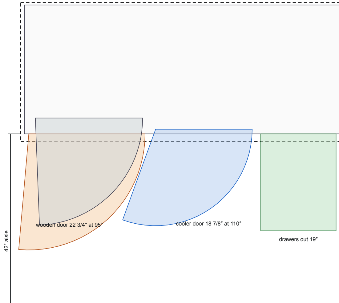
FIGURE 5 OPERATING CLEARANCES: doors, cooler door and drawers open
